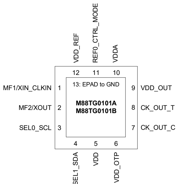
Figure 2. 12-LGA Pin Assignment, 2.5mm x 2.5mm, 0.5mm Pitch (Top view)
