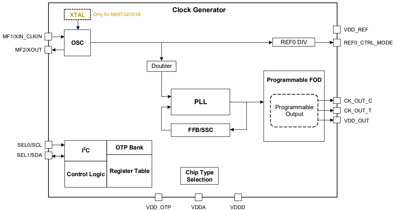
Figure 1. M88TG0101A/B Block Diagram
