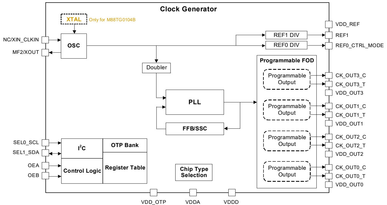
Figure 1. M88TG0104A/B Block Diagram
