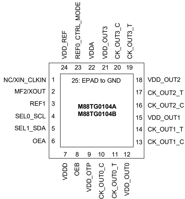
Figure 2. 24-VFQFPN / 24-LGA Pin Assignment, 4.0mm x 4.0mm, 0.5mm Pitch (Top view)
