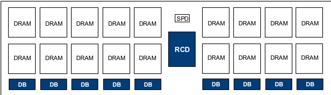
LRDIMM Application Example
