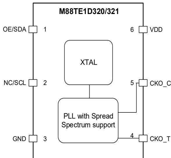
Figure 1. Block Diagram
